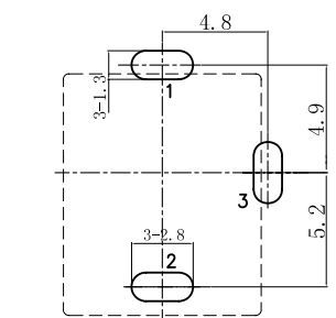
RECOMMENDED PCB LAYOUT TOLERANCE:±0.05mm(TOP VIEW)
